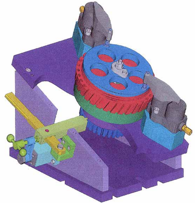
BROACH FIXTURE FOR TURBINE WHEEL MANUALLY INDEXED WITH HYDRAULIC CLAMPING
