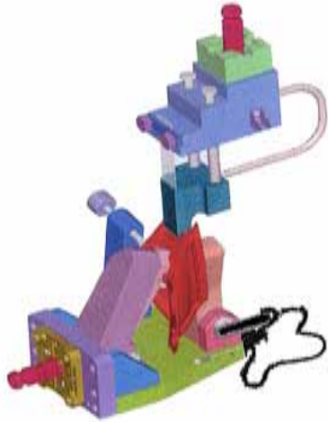
EDM HOLDER AND FIXTURE TO PRODUCE HOLES IN AIRFOIL VANES BOTH FIXTURES AND HOLDER HAVE QUICK CHANGE PALLETS
