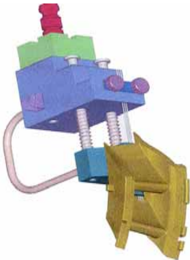
EDM HOLDER AND FIXTURE TO PRODUCE HOLES IN AIRFOIL VANES BOTH FIXTURES AND HOLDER HAVE QUICK CHANGE PALLETS
