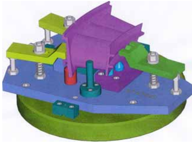
GRIND FIXTURE FOR 5 AXIS
