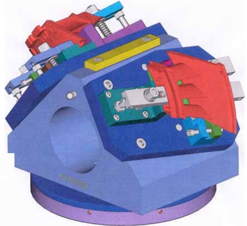
SPLASH GRIND FIXTURE FOR NOZZLE SEGMENTS
